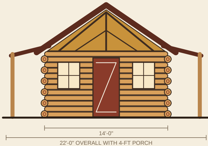
FRONT ELEVATION — SYMMETRICAL GABLE & EXPOSED LOG TRUSS
