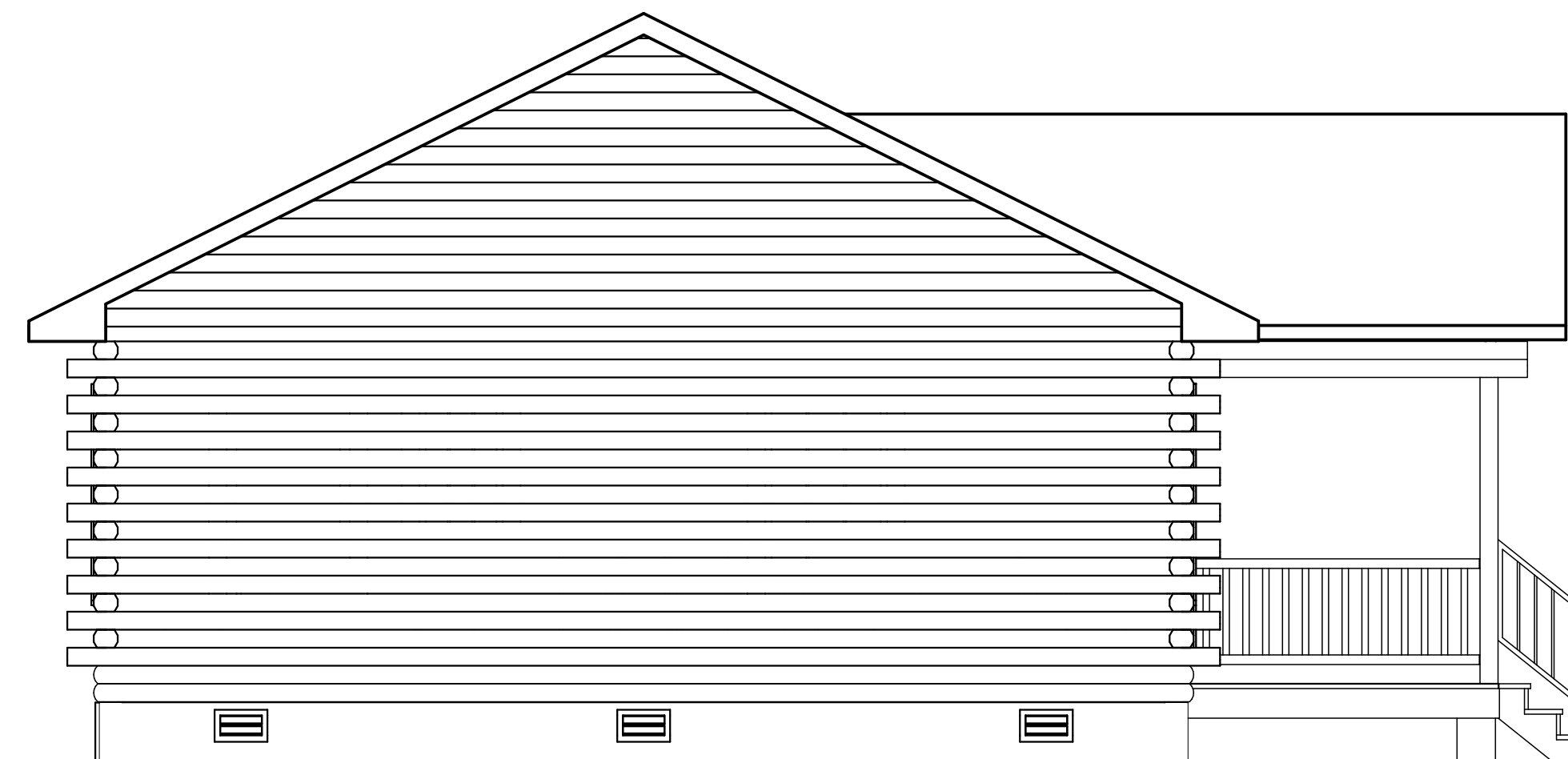
LEFT ELEVATION
