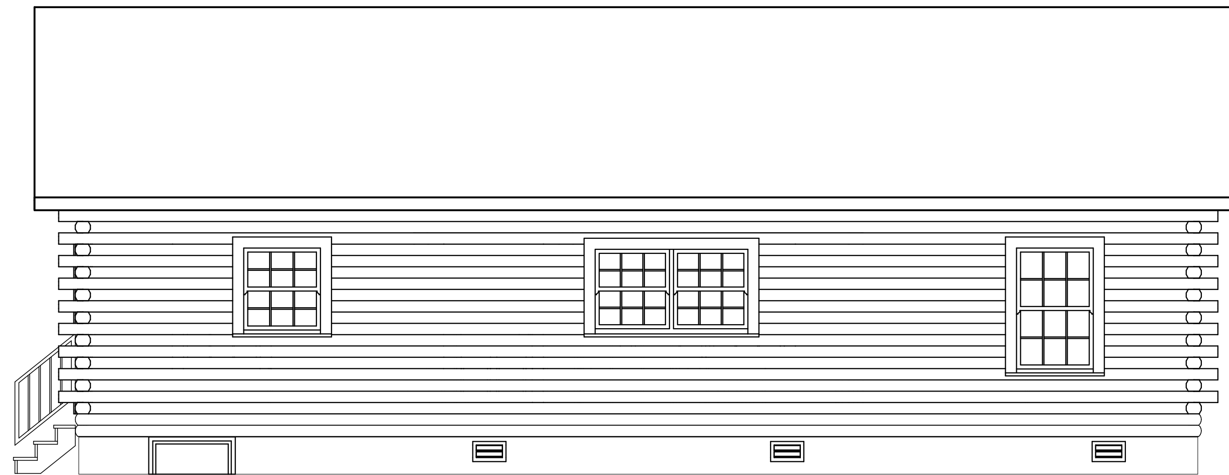
REAR ELEVATION
